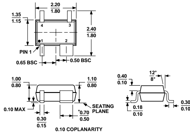
Figure 11. 4-Lead Thin Shrink Small Outline Transistor Package [SC70] (EIAJ SC82 body) (KS-4)
