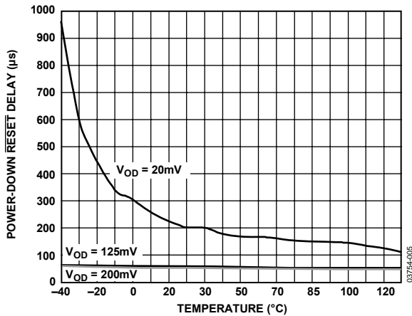
Figure 6. Power-Down \overline{\text{RESET}} Delay vs. Temperature: ADM671_R/S/T/Z
