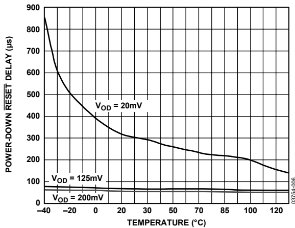
Figure 7. Power-Down \overline{\text{RESET}} Delay vs. Temperature: ADM671_L/M
